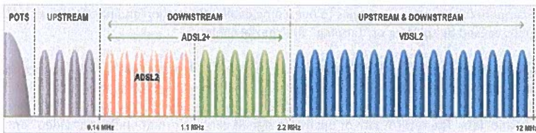
Figure 2: VDSL2+ Frequency Utilization
